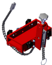
Pipe attachment DMP 251 for pipes with diameters of 80-250 mm (3-10") Product code: PDS-0110-03-00-01-0
